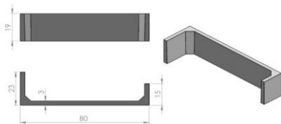
JPSM07 - Shaft Modular® 80 (80 x 23/15 x 19)
