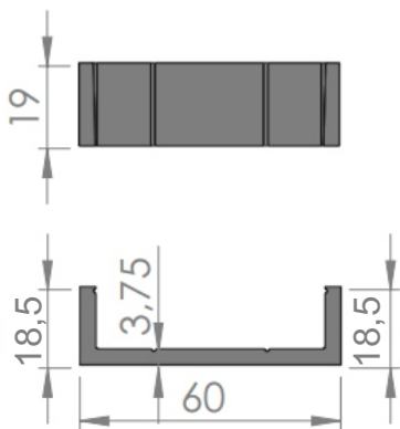
JPSM03 - Shaft Modular® 60 (60 x 18,5 x 19)
