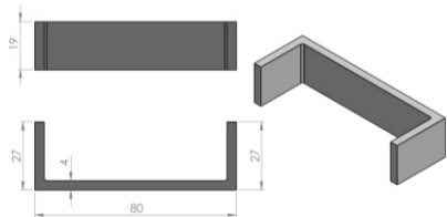
JPSM05 - Shaft Modular® 80 (80 x 27 x 19)
