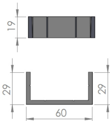
JPSM03 - Shaft Modular® 60 (60 x 29 x 19)
