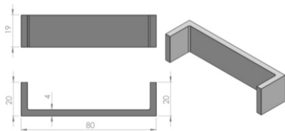
JPSM04 - Shaft Modular® 80 (80 x 20 x 19)
